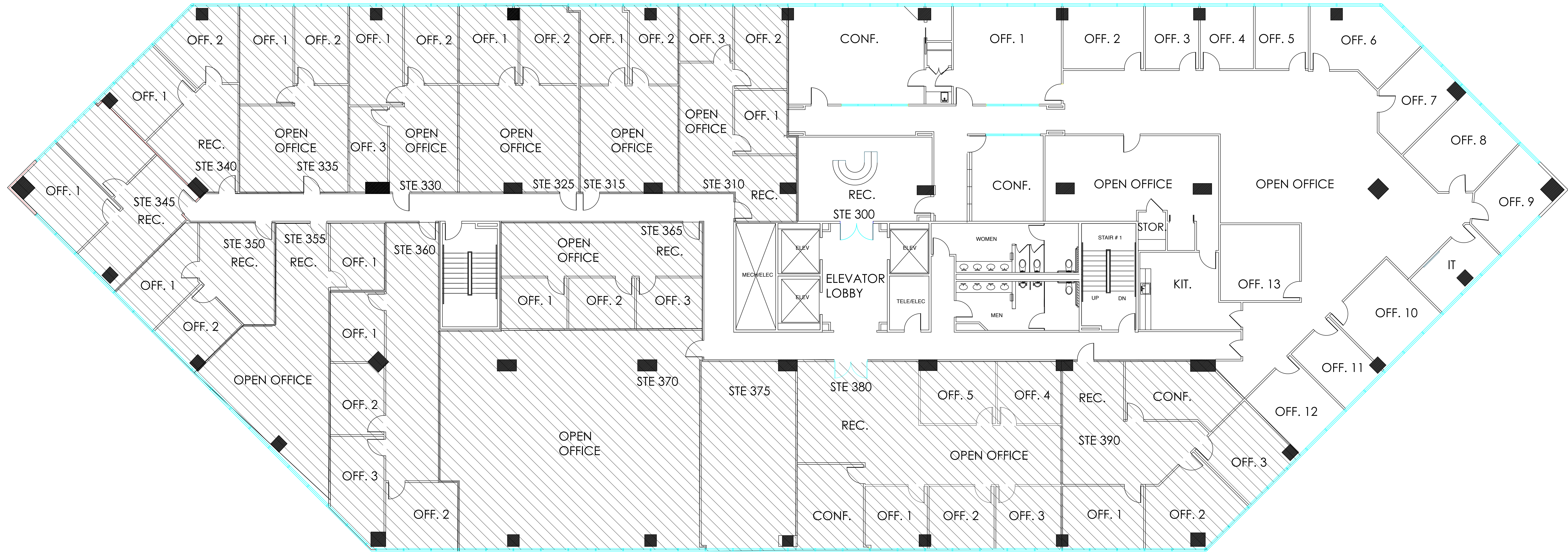
03 | L - 3 FLOOR PLAN SUITE 300 8,017 sq. ft. SCALE: 1/8" = 1'-0"
